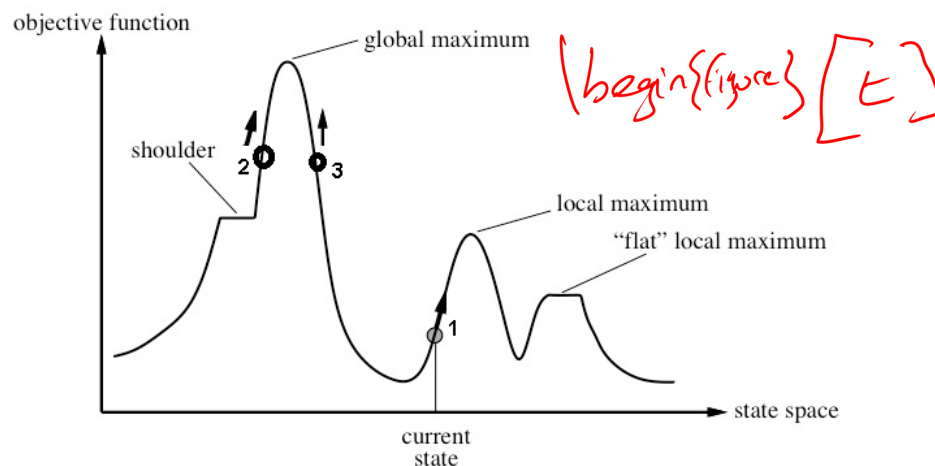
Figure 2.6 Hill Climbing Algorithm
