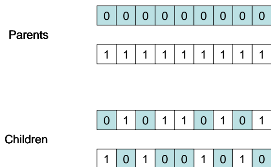
Figure 2.4 Uniform Crossover
