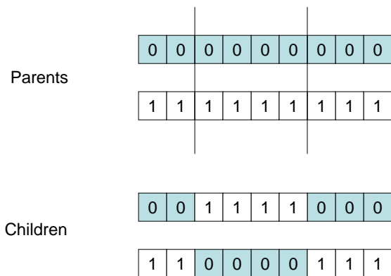
Figure 2.3 Two-Point Crossover
